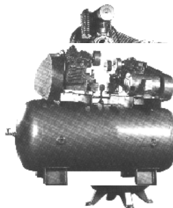
MODEL X755-120 10 hp. duplex 120 gallon tank
